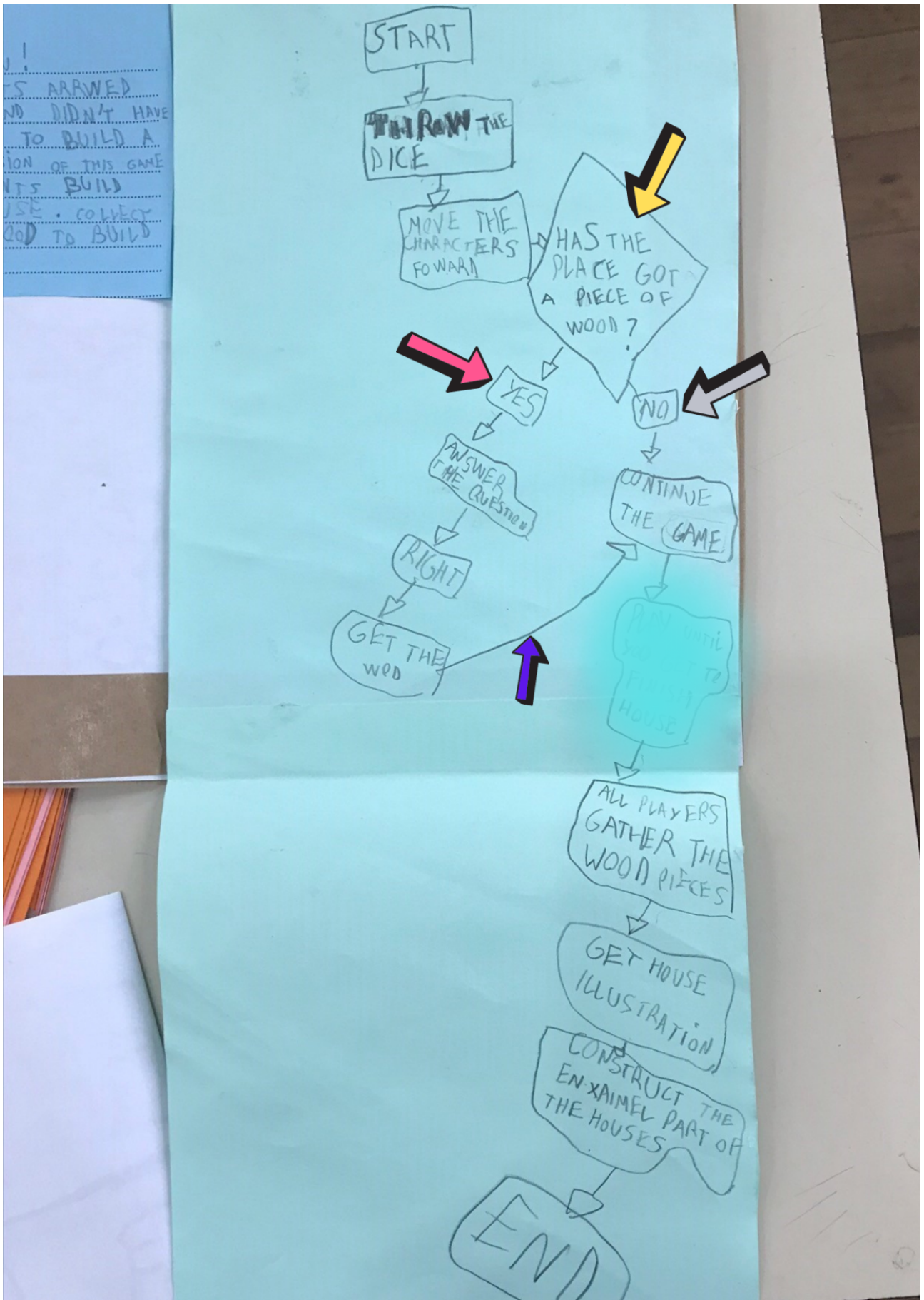
Image 3. Conditional Structures
